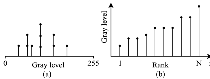
Fig. 8. Histogram and vector: (a) the histogram of the gray levels of one of the subwindows, and (b) the vector of the rank-ordered gray levels of one of the subwindows plotted against the rank i ( i = 1, \dots, N ).
